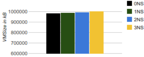
Fig. 12. Average memory footprint in kB (VmSize) for 0-, 1-, 2- and 3-namespaces configurations.
