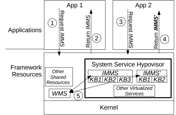
Fig. 7. PINPOINTing InputMethodManagerService .
