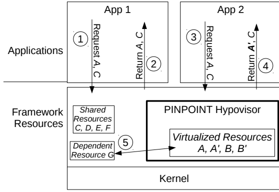
Fig. 1. PINPOINT concept showing minimized isolation to address security goals, with maximized sharing of system objects.
