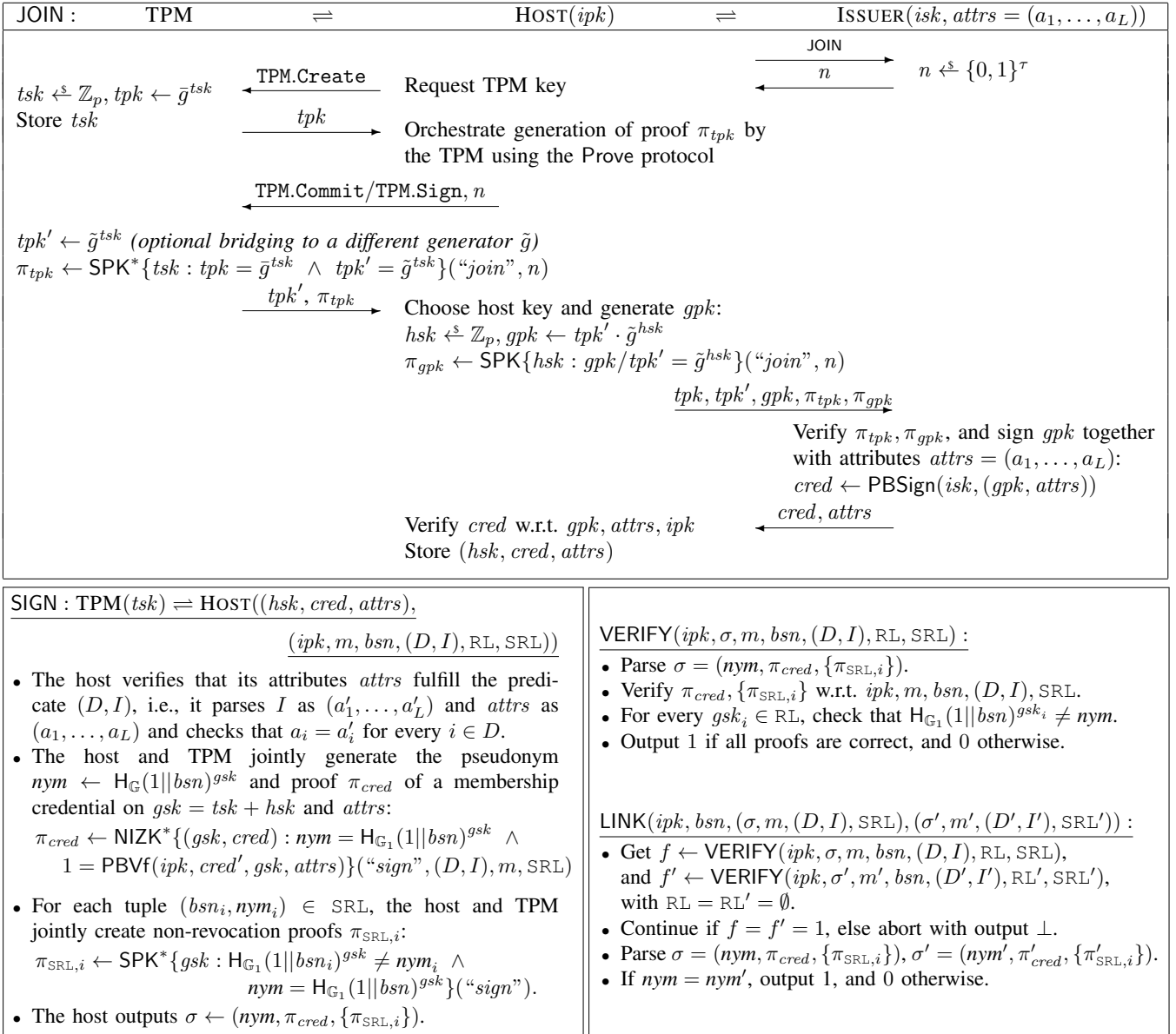
Fig. 4. High-level overview of the DAA protocols.
