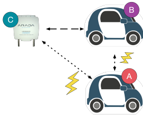
Fig. 3. False Alert Attack Scenario
