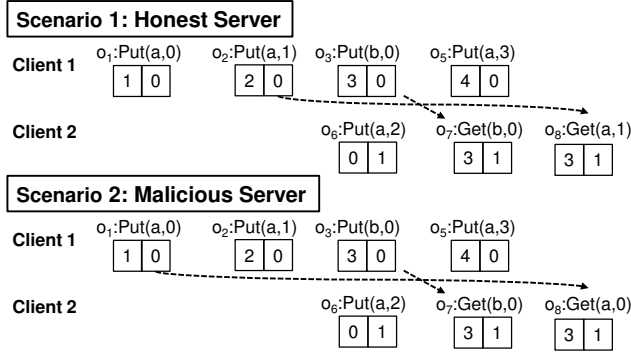
Fig. 4. Verification of causal consistency. The vector clock is shown below each operation as \begin{bmatrix} C1 \\ C2 \end{bmatrix} .
