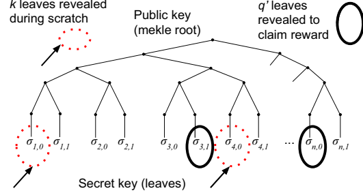
Figure 3: Illustration of the floating preimage signature scheme.
