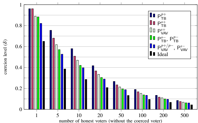
Fig. 4. Level of coercion ( \delta ) for different protocols with two candidates, p_0 = 0.3 , p_1 = p_2 = 0.35 . The goal of the coerced voter is to vote for candidate 1.
