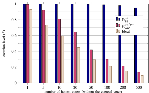
Fig. 5. The lower-bound of coercion-resistance ( \delta ) for ThreeBallot in the variant by Marneffe et al. and the precise values for VAV in the privacy enhanced variant and the ideal voting protocol with 10 candidates, where an honest voter abstains from voting with probability p_0 = 0.3 and she chooses a candidate with probability ((1 - p_0)/10) .
